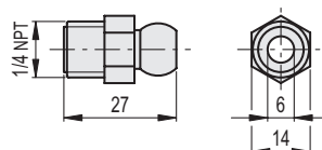
FHJ.1/4-1/4-NPT
